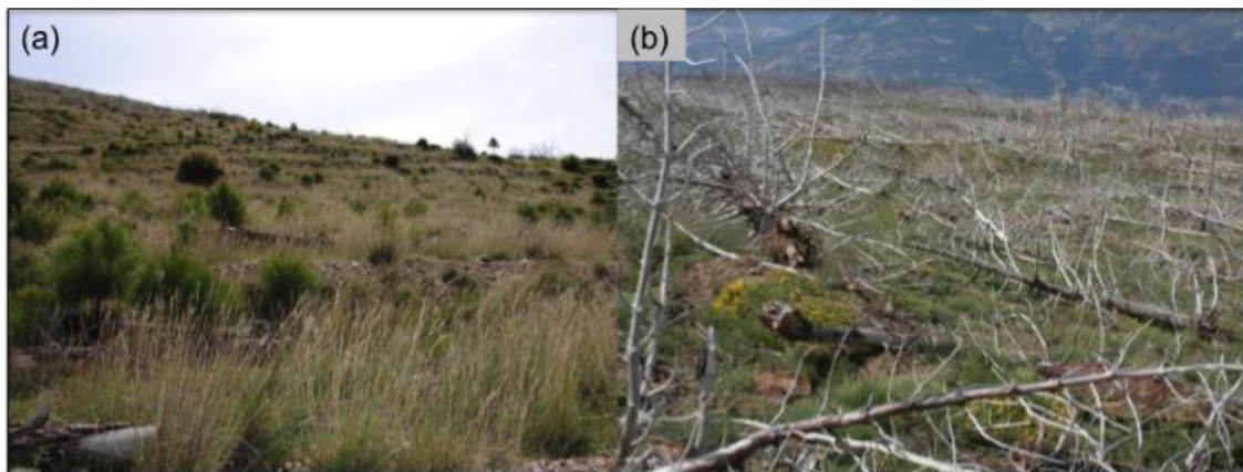
Fig. 1. Photographs of the burnt-wood management treatments: (a) Salvage Logging, and (b) Non-Intervention. The fire occurred in September 2005, treatments were implemented in spring 2006, and the photos are from 2012. Photo (a) courtesy of R. Marzano, photo (b) by JC.
