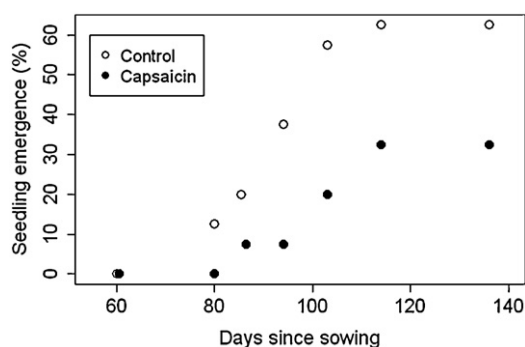
Fig. 4. Percent seedling emergence with and without the application of capsaicin. The acorns were sown in plastic containers and isolated from predators, and emergence was monitored.
