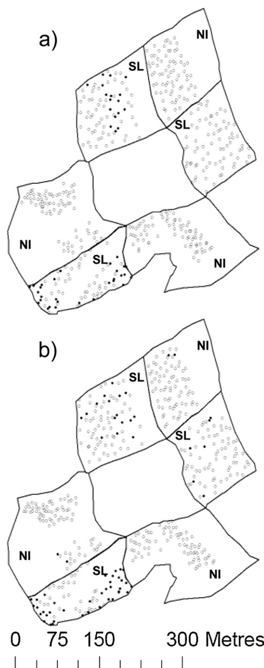
Fig. 3. Spatial distribution of predated (grey points) and non-predated (black points) acorns sown at (a) 2 cm and (b) 8 cm depth in 2010. Post-fire treatments are Salvage Logging (SL) and Non-Intervention (NI).
