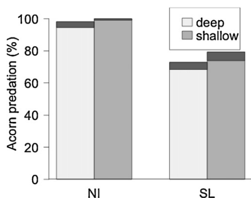
Fig. 2. Percent acorn predation in the Non-Intervention (NI) and the Salvage Logging (SL) post-fire management treatments in 2010. Graphs show differences between deep (8 cm) and shallow (2 cm) buried acorns for both treatments. The dark grey areas on the upper part of the bars indicate predation by boars, and the lower part by rodents. Note that mean differences between deep and shallow acorns were larger in the SL than in the NI treatment.
